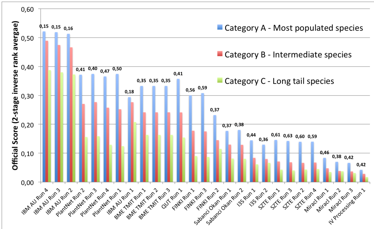
Figure 7: PlantCLEF results detailed by ordinarieness categories
