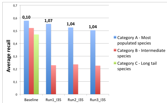
Figure 8: FishCLEF results detailed by ordinariness categories
