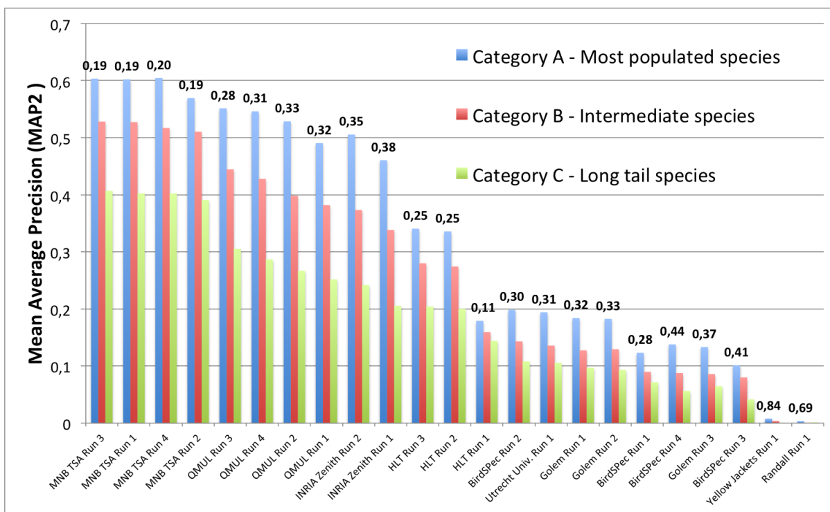
Figure 6: BirdCLEF results detailed by ordinariness categories
