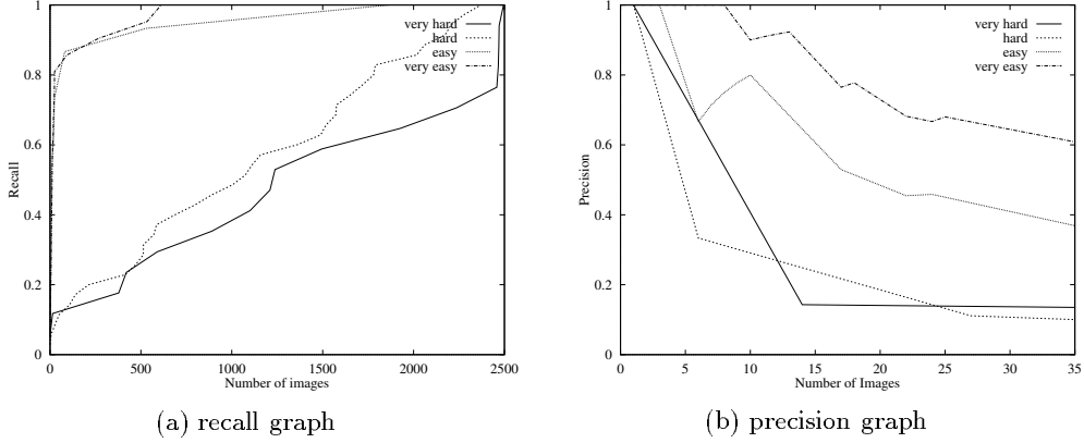
Figure 2: Recall vs. No. of images graph and partial precision vs. No. of images graph
