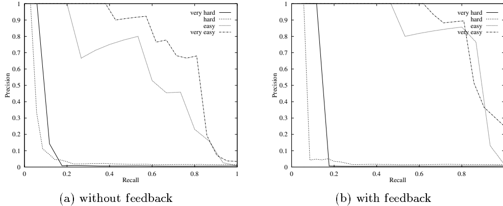
Figure 1: PR graphs for four different queries both without and with feedback.
