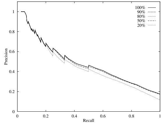
Figure 5. Precision vs. recall when evaluation is stopped after a fixed percentage of features.
