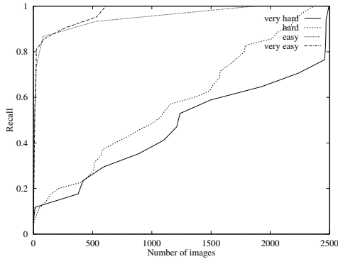
(a) recall graph
