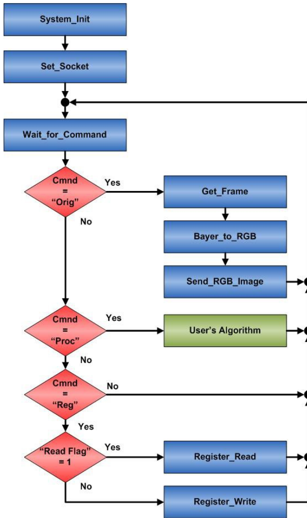
Figure 4. Block diagram of code architecture.
