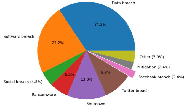
Fig. 6: Attack distribution
