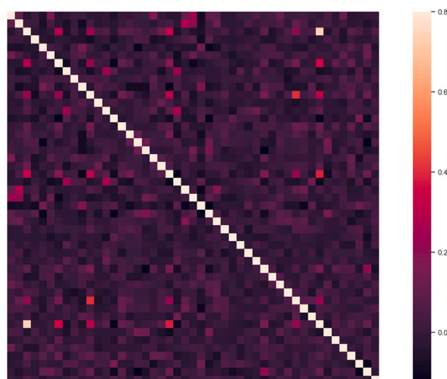
Fig. 7. Correlation of residuals. Correlation matrix of residuals, obtained by estimating Eq. (1).
