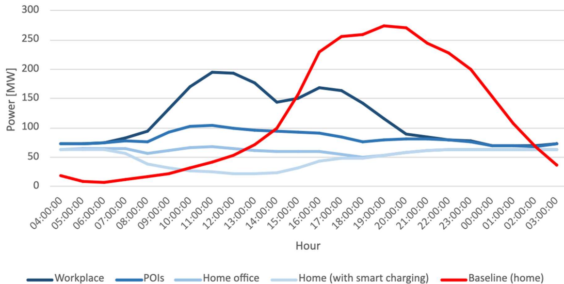
Figure 5: Load curves of EV charging obtained for the Baseline and Scenario C
