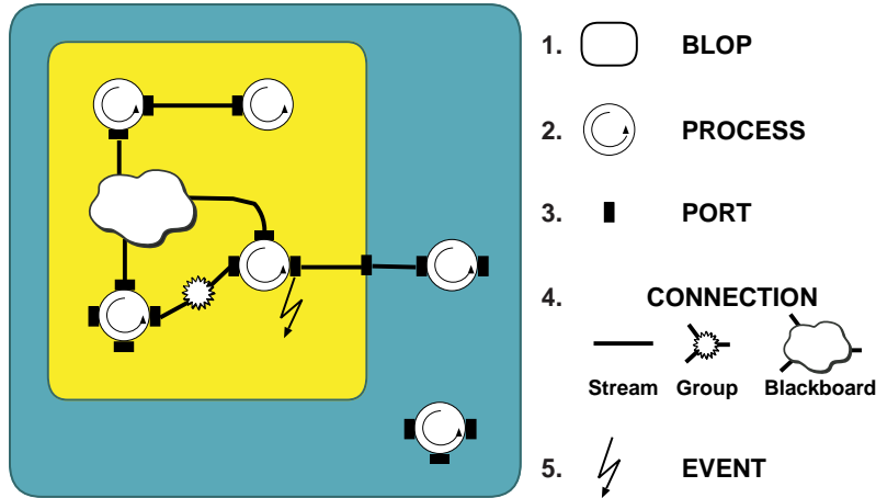
Figure 4.1: The ECM coordination model.
