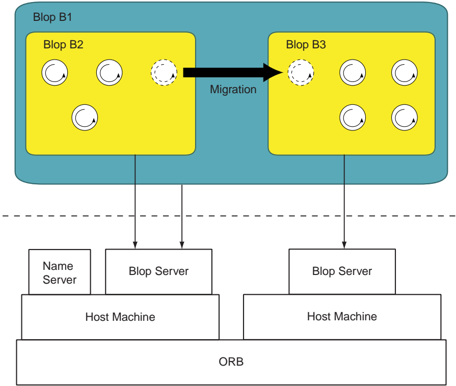
Figure 7.2: The ORB integration of AGENT&Co.
