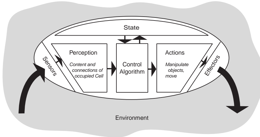
Figure 2.6: Our target agent architecture.
