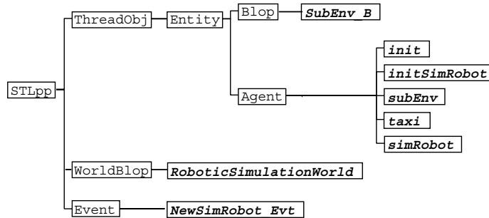
Figure 8.3: Robotic Simulation class hierarchy.
