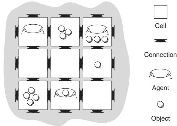
Figure 2.5: Generic MAS Model.
