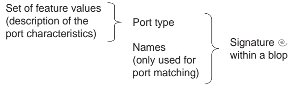
Figure 4.2: Signature of a port.
