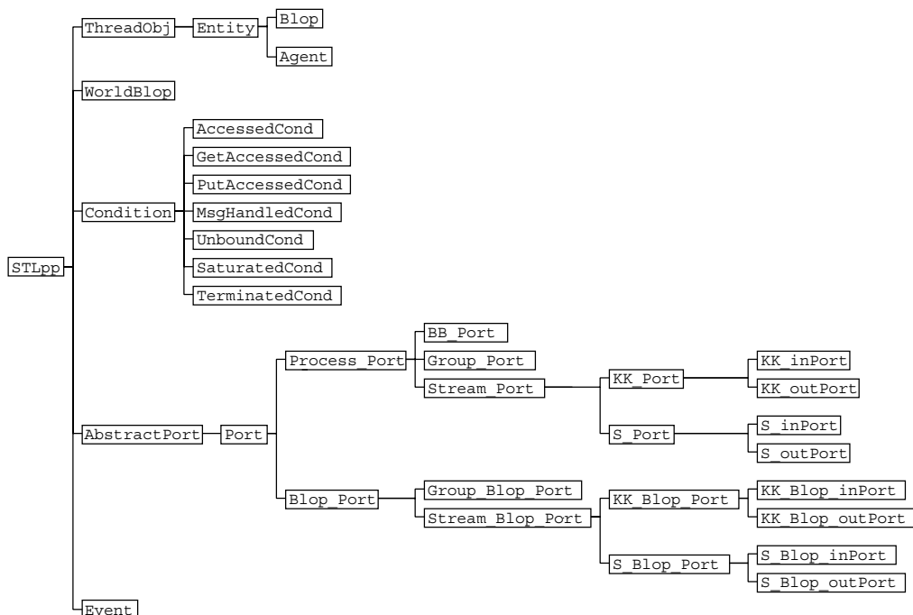
Figure 6.2: STL++ user classes.
