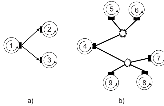
Figure 6.9: Ports with multiple connections: a) stream b) group.
