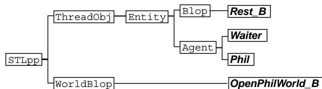
Figure 6.13: Classes of the dining philosophers program.
