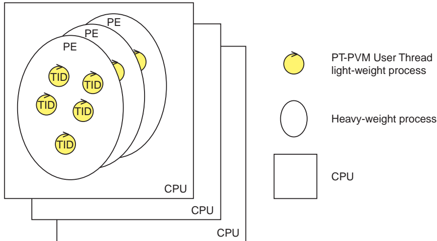
Figure 6.18: PT-PVM programming abstractions.
