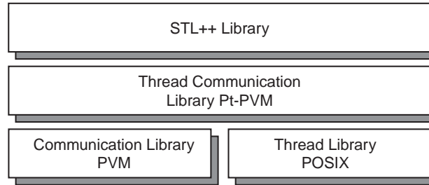
Figure 6.17: Overview of the implementation layers of STL++.
