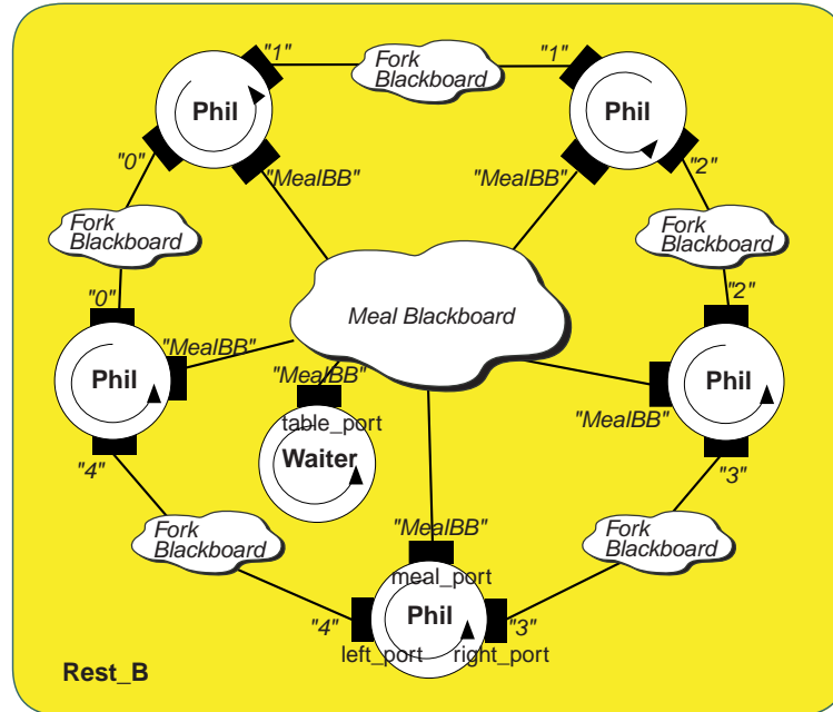
Figure 6.12: Dining philosophers implemented with STL++.
