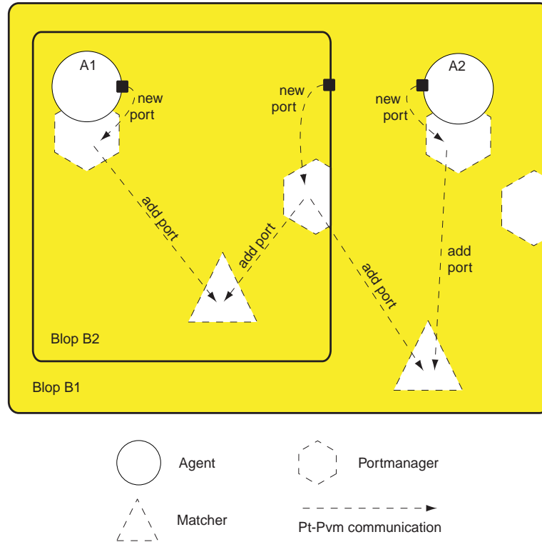
Figure 6.19: Implementation of the matching mechanism of STL++.
