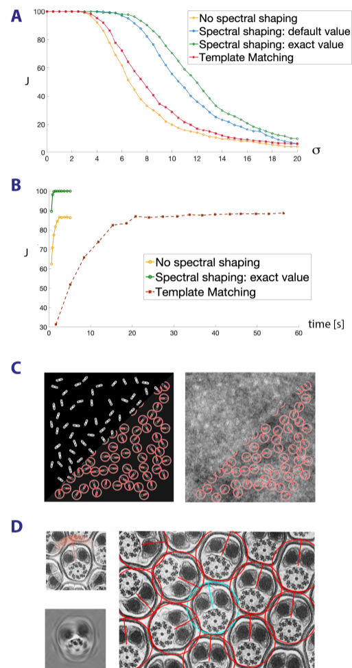
Fig. 1. A Performance comparison of template matching, adapted steerable filters (no spectral shaping), and Steer'n'Detect with \gamma = 1 (optimal) and \gamma = 0.5 (suboptimal), measured by the Jaccard index J as a function of the amount of background noise (standard deviation \sigma ). B Performance comparison of rotated template matching, adapted steerable filters (no spectral shaping), and Steer'n'Detect, measured by the Jaccard index J as a function of run time, for a fixed background signal ( \sigma = 5 ). C Detection of rod-shaped bacteria with Steer'n'Detect (synthetic image degraded by self-similar Gaussian random field background noise). D Detection of spermatozoan axoneme with Steer'n'Detect (transmission electron microscopy image). Top left: image crop used as template; bottom left: resulting detector; right: detection results.
