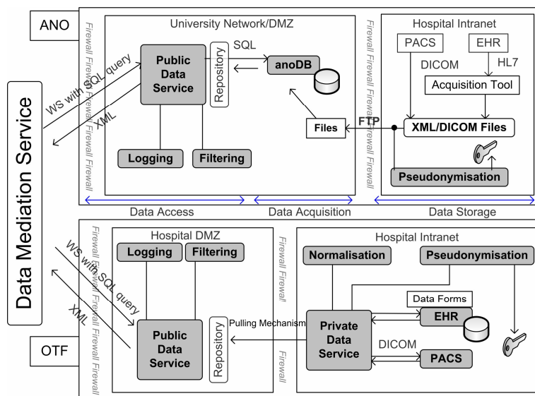
Figure 2: ANO and OTF architectural solutions
