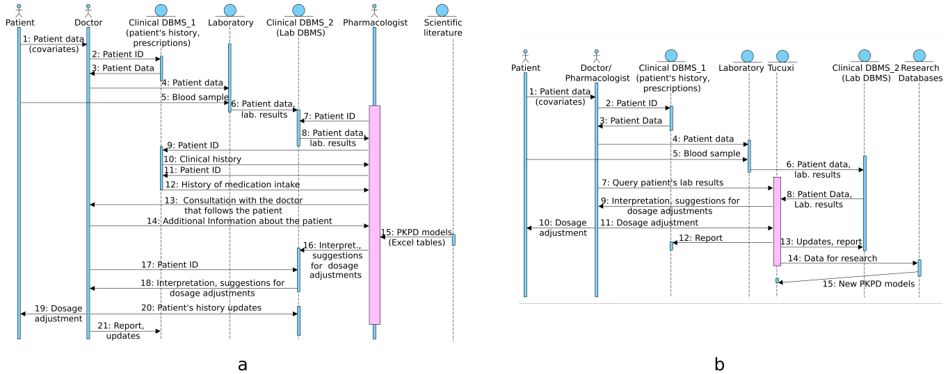
Figure 1: TDM in clinical practice: non-automatized process (a), TUCUXI (TDM software) integrated in clinical practice (b).
